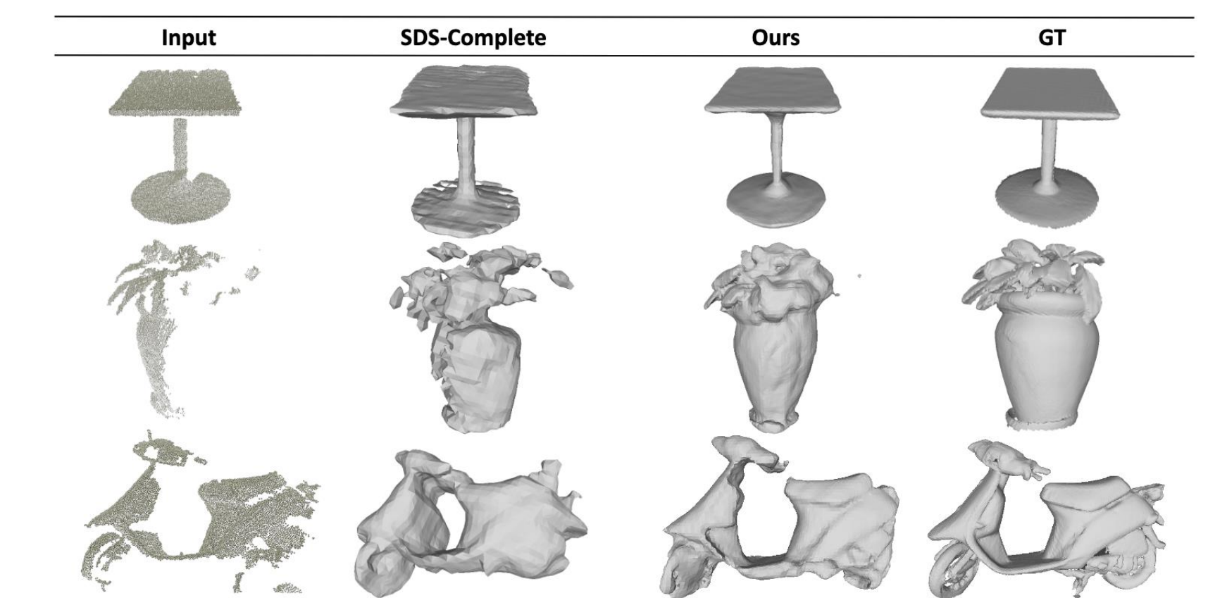
Comparisons based on the Mesh Completion.
