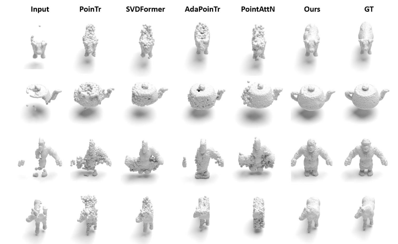
Comparisons on the completion of synthetic data.
