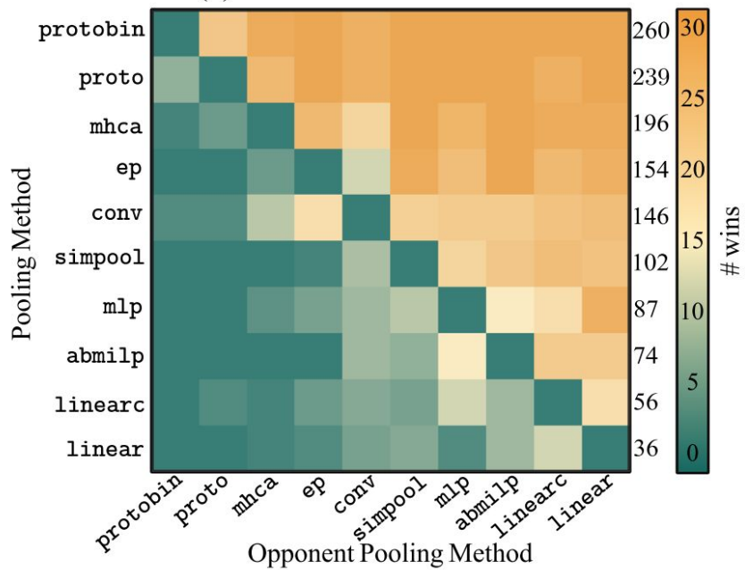
(a) General multi-label audio
