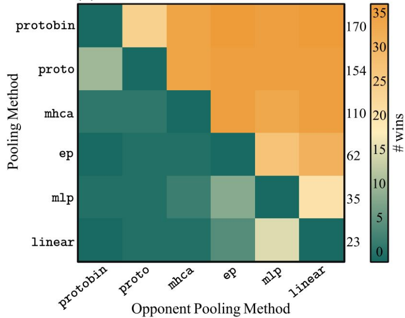
(b) Few-shot multi-label bioacoustic
